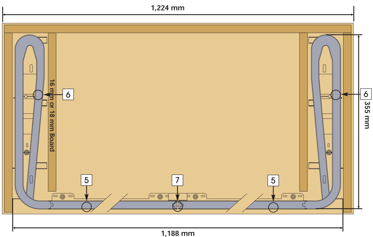
■ Bottom View: Parts & layout of Roller Shutter Tracking System.
