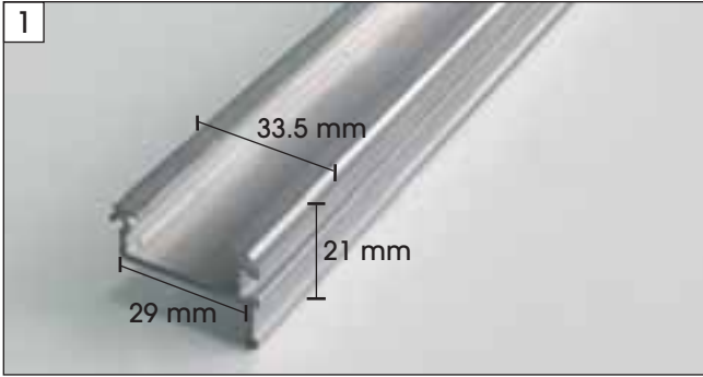
Item Code : SW 721 Aluminium Profile
