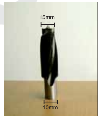
Boring Bit for Minifix-Housing
