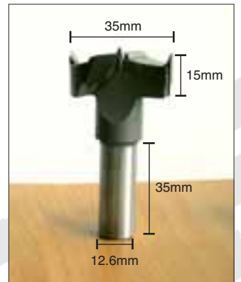
Router Bit for Steel Hinges 35mm Wire Cap
