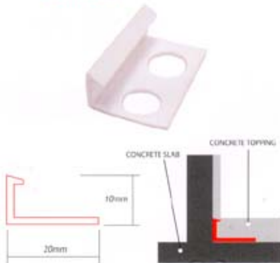
MJ1 FLOOR/WALL EXPANSION MOVEMENT JOINT, PERIMETER EXJI.B01.1
