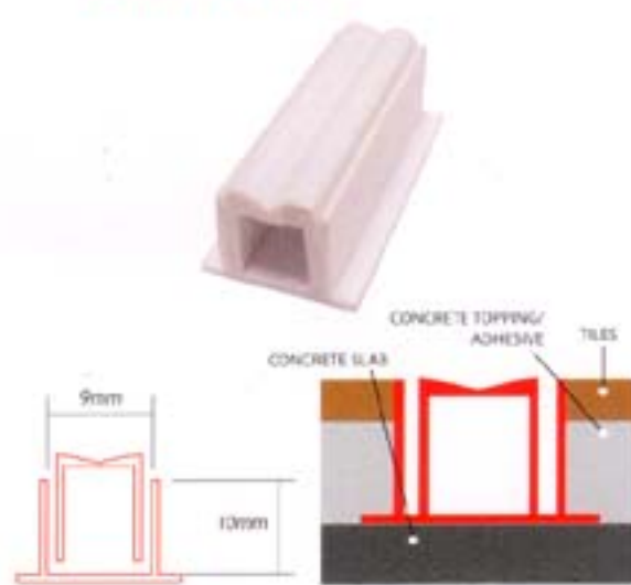
MJ2 FLOOR EXPANSION MOVEMENT JOINT, PERIMETER EXJI.A01.1000
