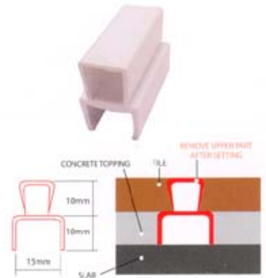
MJ3 FLOOR TOPPING GUIDE FTG1.A01
