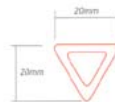
GT1 PLASTERING GUIDE TRIANGULAR 20MM PLGI.K01
