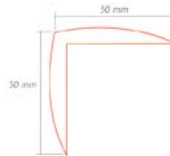
PG1 PARKING GUARD / POST PROTECTOR FIT2.A019.31
