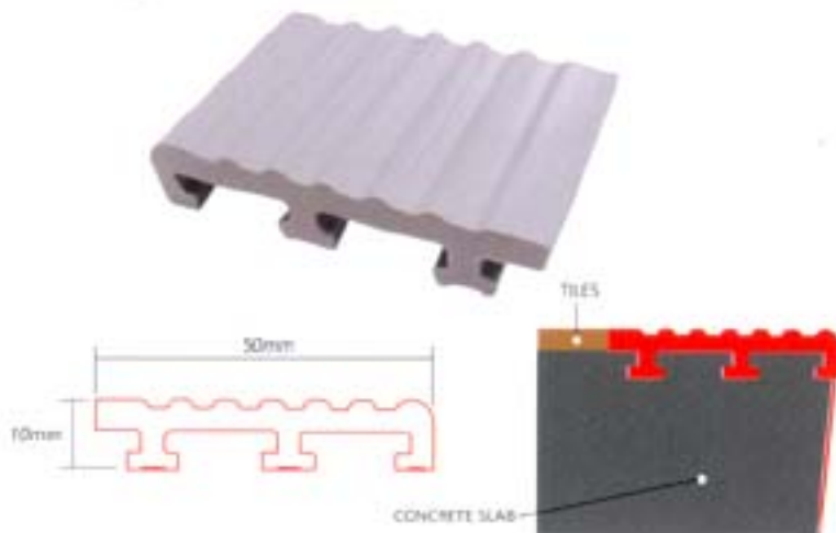
SN1 STAIR NOSING RIGID 50MM STN.B
